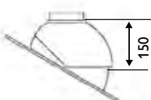
F11 - pitched roof flashing
